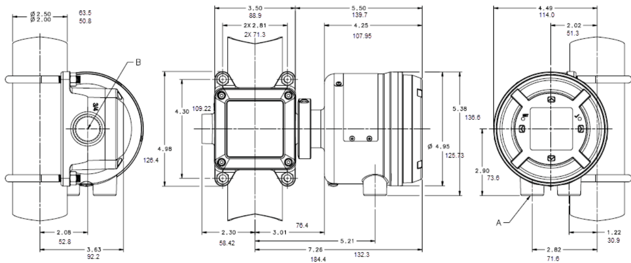
Figure 2: Remote mount transmitter
