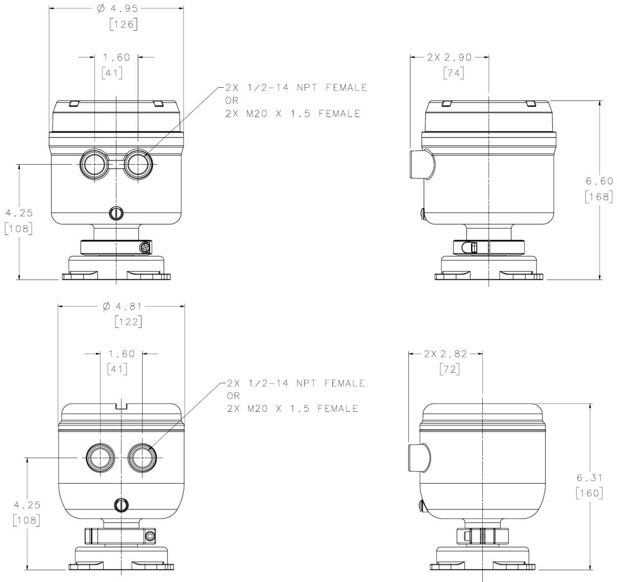
Figure 4: Integral mount transmitter with retrofit adapter
