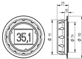
Panel mounting
