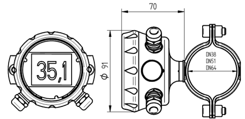
Tube mounting
