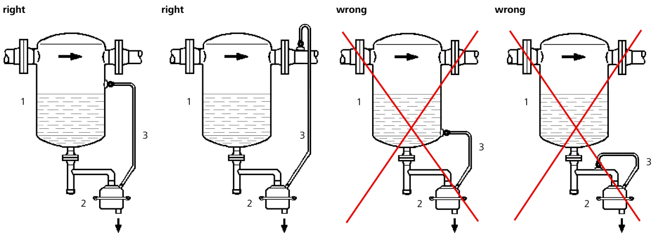
1 condensate collection tank 2 condensate trap 3 compensation line use MANKENBERG-products
