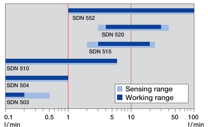
Flow ranges for EGE-Inline-Compact models
